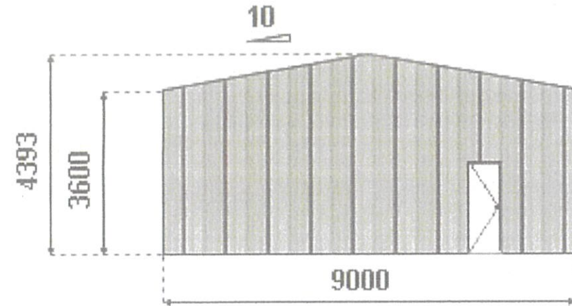
EASTERN ELEVATION Back
