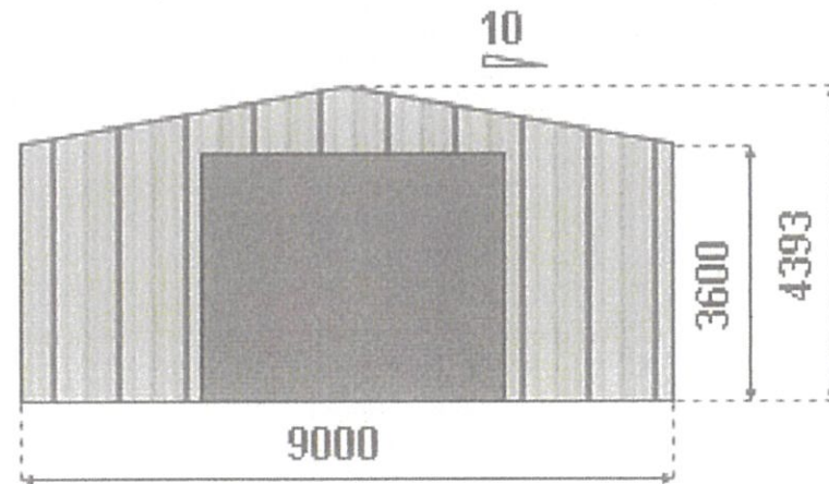
WESTERN ELEVATION Front
