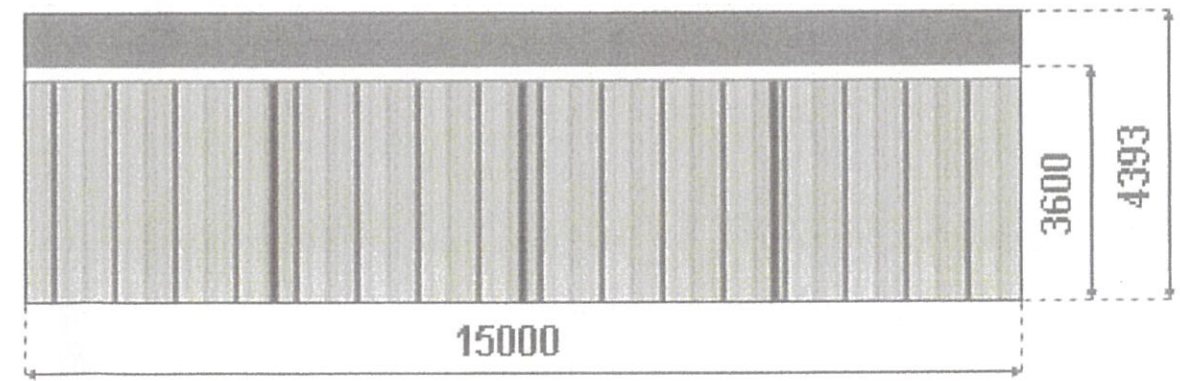
SOUTHERN ELEVATION Right
